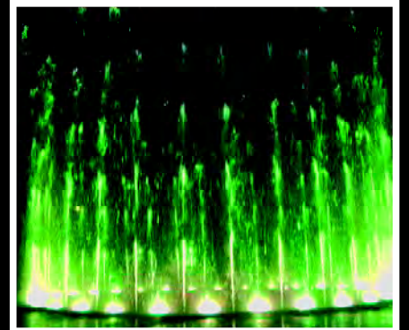
Palm Beach Zoo Musical Fountain & Spray Apron , Palm Beach , Florida, USA PEM W 115-5 Water Switches, PEM 846 Jets, PEM C 133-4 Multi Colored Submersible Lights
